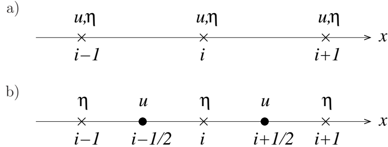
Figure 1.2: A regular grid with the gravity wave variables u and \eta co-located on an non-staggered grid (a) and on a staggered grid (b).
