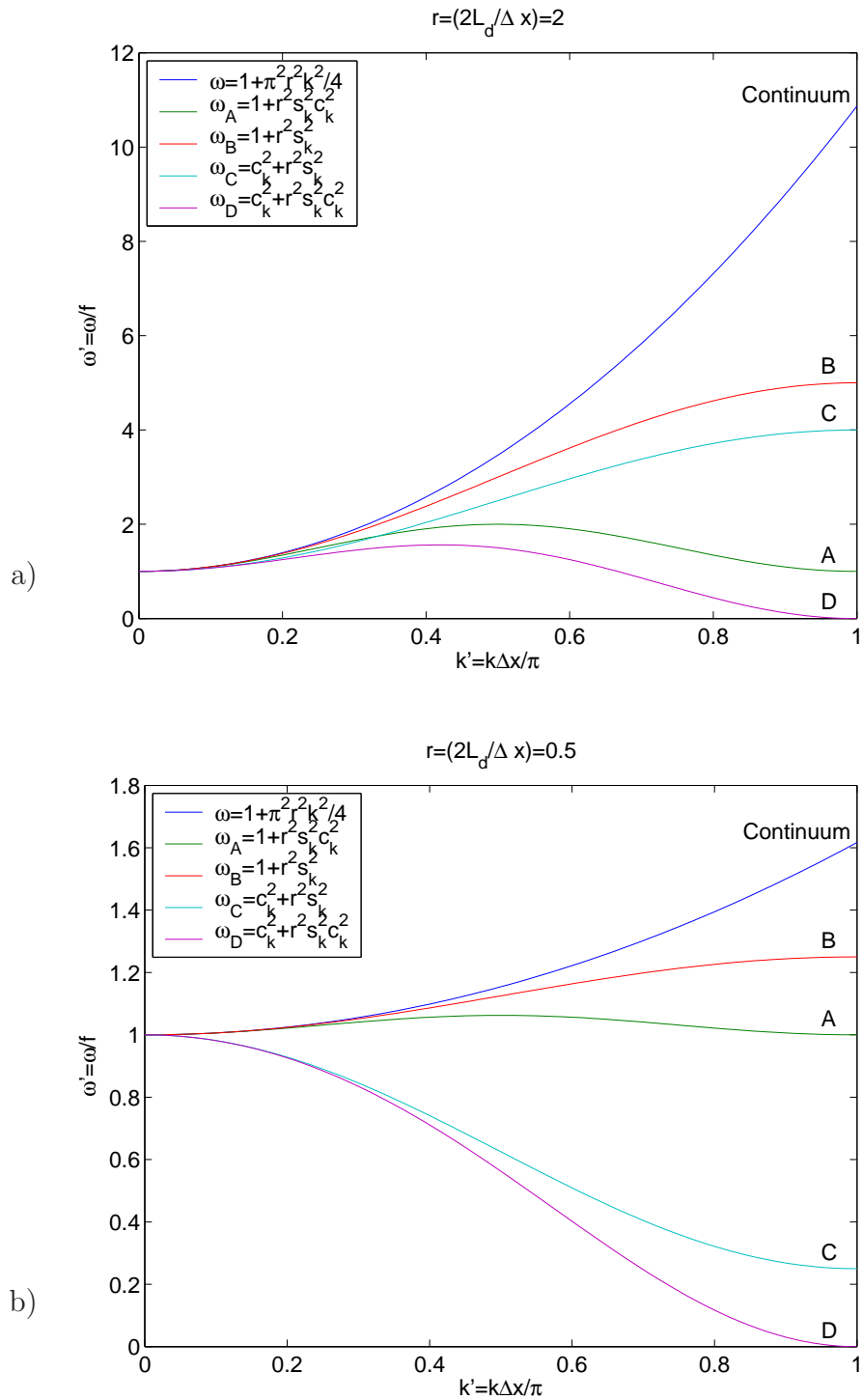
Figure 1.5: The one dimensional dispersion relations for inertia-gravity waves in the continuum and for the four grids, (A, B, C and D) for (a) r = 2 and (b) r = 1/2 .
