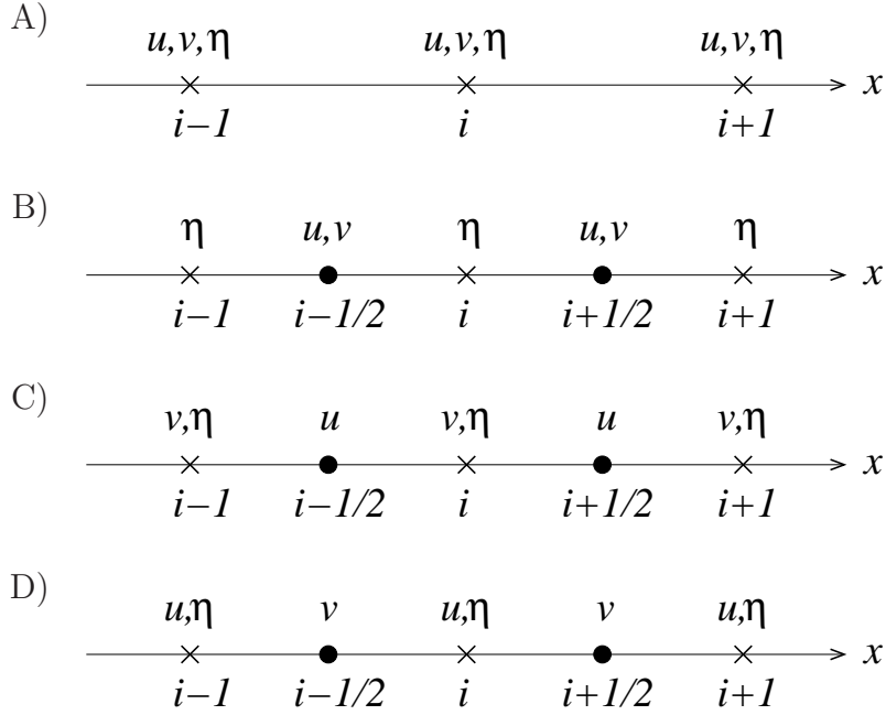
Figure 1.4: The inertia-gravity wave variables u , v and \eta in the four possible configurations (A, B, C and D) on a finite difference grid.
