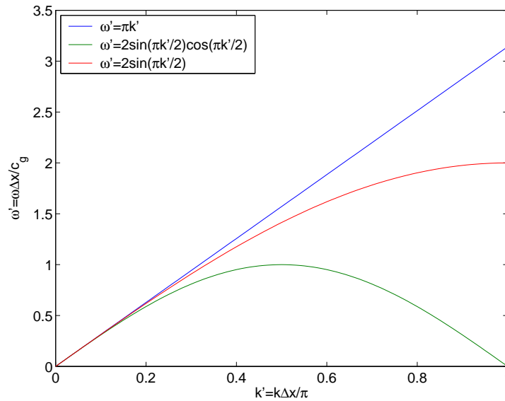
Figure 1.3: Dispersion of numerical gravity waves for the non-staggered grid (green) and the staggered grid (red). The continuum ( \omega = k ) is plotted for comparison (blue).
