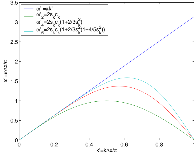
Figure 1.1: Dispersion relations for constant flow advection in the continuum, and using second and fourth order spatial differences.
